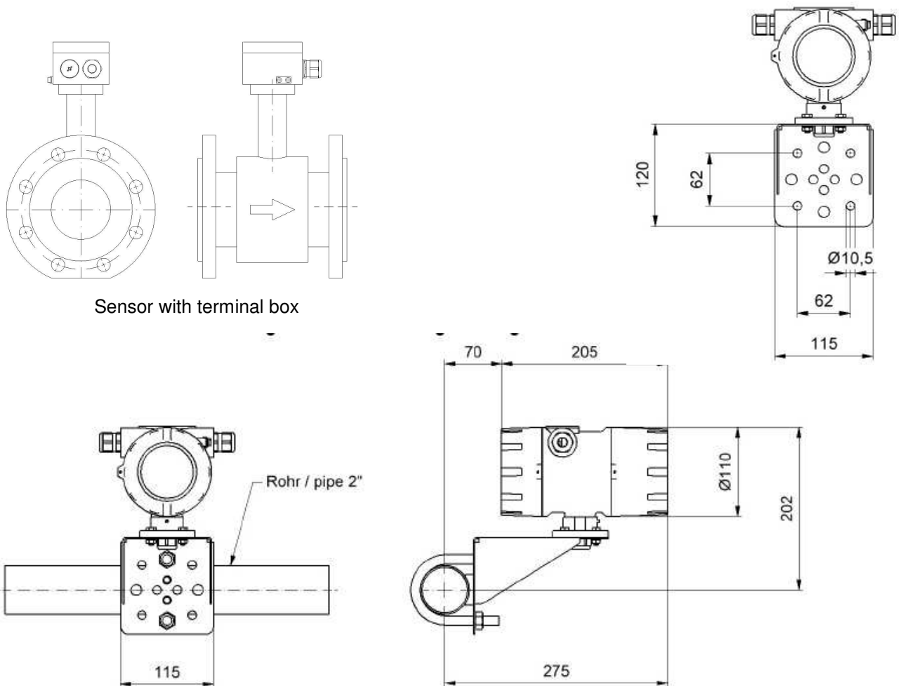
Transmitter with wall / pipe mounting bracket
