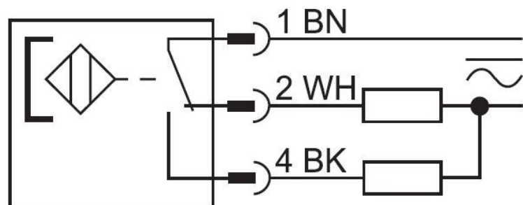
Figure 3: Electrical connection GSGW
