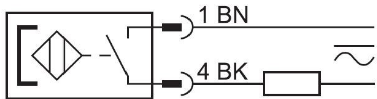
Figure 2: Electrical connection GSGB
